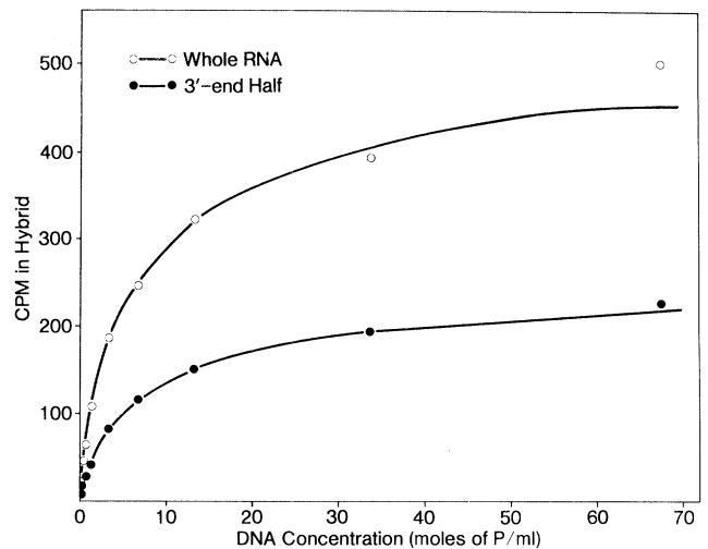
FIG. 1. Dependency of hybridization level on DNA concentration. 125 I-Labeled, whole \kappa mRNA of MOPC 321 (1300 cpm) or its 3'-end half fragment (600 cpm) was annealed with varying indicated amounts of denatured MOPC321 DNA in 0.3 M NaCl, 0.03 M sodium citrate (pH 7) at 70° for 42 hr. The volume of annealing mixture was 0.05 ml. Specific activity of the RNA was 6.5 \times 10^7 cpm/µg. Each point represents an average of duplicate measurement. Intrinsic RNase-resistant counts, 22 cpm for whole RNA and 16 cpm for 3'-end half, are subtracted.
