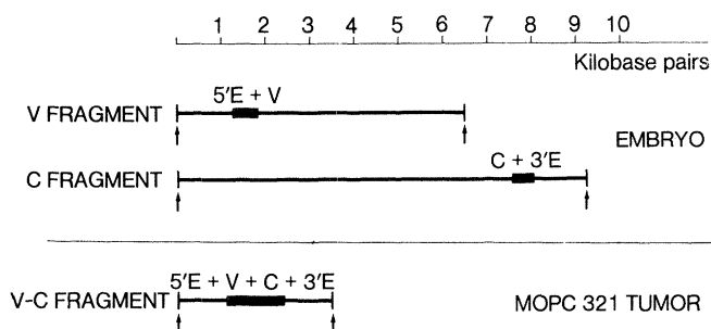
FIG. 3. Mouse DNA fragments carrying V_{\kappa} and C_{\kappa} genes. DNA fragments were generated by Bam H I restriction endonucleases. Arrows indicate Bam H I sites. 5'E and 3'E designate base sequences corresponding to untranslated regions of a \kappa -chain mRNA molecule at the 5'- and 3'-end, respectively. V and C designate base sequences corresponding to variable and constant regions, respectively. The relative position of these sequences within each fragment is deduced from the present results within the framework of either of the latter three models depicted in Fig. 4.
